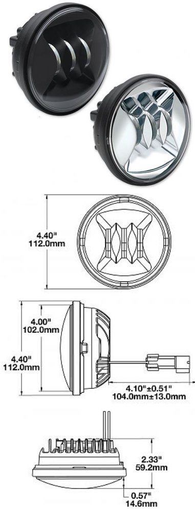
Dimensions in inches (mm in parentheses). Dimensions are for reference only.
