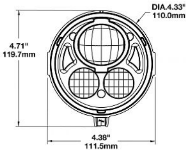
Model 8415 High/Low and Low Beam Only LED Headlights, LED head lights, LED headlamps, LED head lamps
